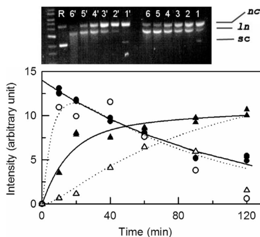
Figure 9. Time course (10, 20, 40, 60, 90, 120 min, lanes 1–6 and 1'–6', respectively) of plasmid cleavage by Cu II -P1 in the presence of 1.0% H 2 O 2 (lanes 1–6, 50.0 \mu M RU; ●, nc form; ▲, ln form; and theoretical fittings, solid traces) and by free Cu II /H 2 O 2 (50 \mu M, lanes 1'–6'; ○, nc form; △, ln form; and theoretical fitting, dotted traces) at pH 8.0 and room temperature, stained with ethidium bromide. The standard DNA ladder starts with 1 kbp from the bottom with 1 kbp increment upward. R is the plasmid DNA pQE30Xa of ca. 3.5 kbp without treatment. The data are fitted with the kinetic models discussed in the text.
